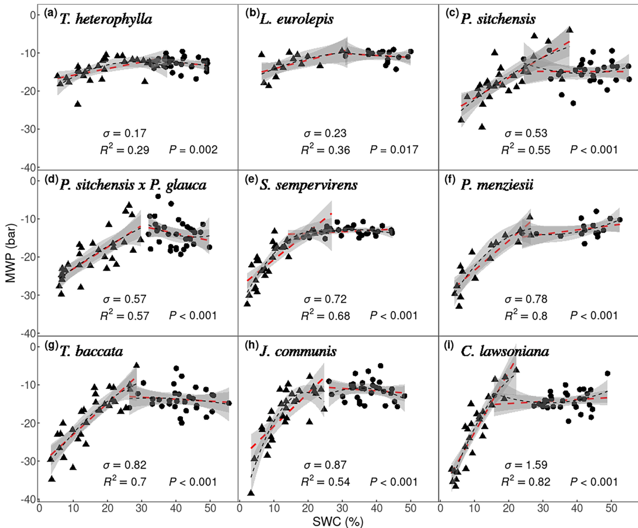
Fig. 4. Curvilinear and linear relationships between MWP and SWC. Circles: well-watered controls, N = 16\text{--}32 ; triangles: drought-treated trees, N = 16\text{--}32 . Red line: Linear regression model of MWP against % SWC. Black dashed line: second order polynomial regression. R^2 , P -values and slope for the ordinary linear model for drought-treated trees are shown. Grey areas are 95 % confidence intervals.
